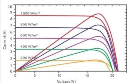
I-V characteristics at different irradiations
