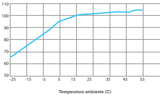
Capacity maintenance (%)
